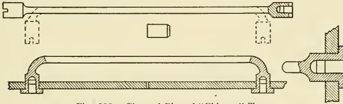
Fig. 205. Channel Pins of "Chicago" Type
